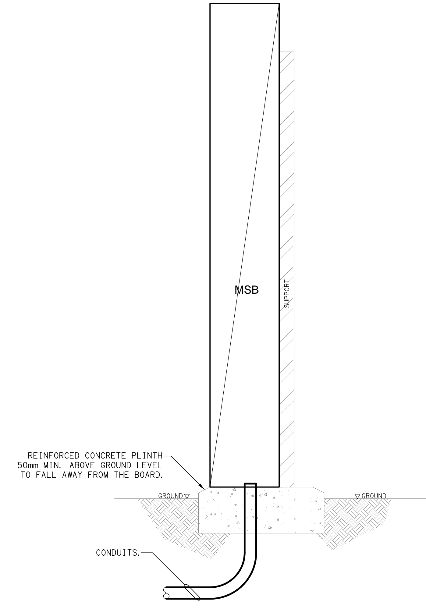
DETAIL MSB MOUNTING SECTION NOT TO SCALE
